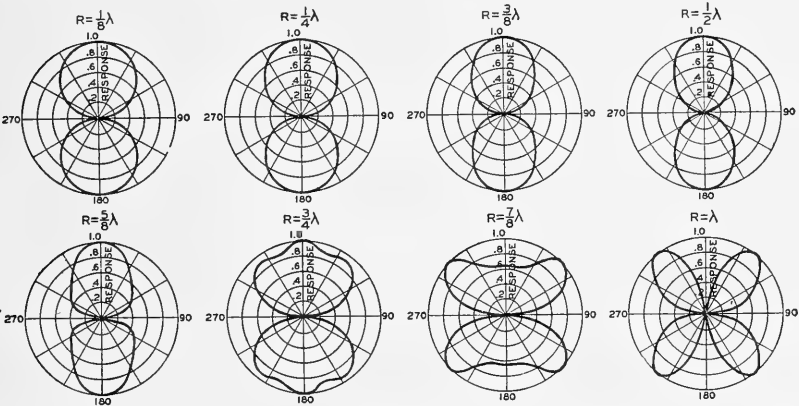
FIG. 9.21. Computed directional characteristics of a ribbon microphone with a large circular baffle (see Fig. 9.17) as a function of the radius of the baffle and the wavelength. The polar graph depicts the output, in volts, as a function of the angle, in degrees. The maximum response is arbitrarily chosen as unity.
